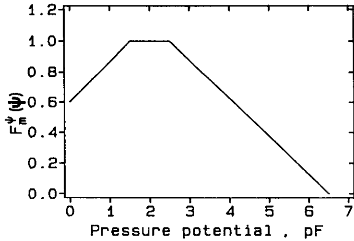
Fig. 6-5 Pressure potential function for adjustment of decomposition rate coefficient to actual soil water pressure potential.
