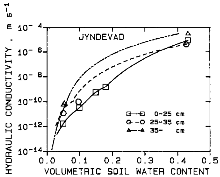
Fig. 11-3 Hydraulic conductivity functions for Jyndevad soil.
