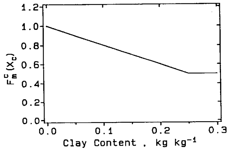
Fig. 6-2 Clay content function for adjustment of the decomposition rate coefficient to actual clay content.
