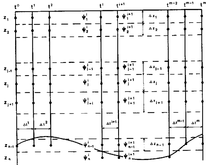
Fig. (4-1) Discretization after the finite difference method.
