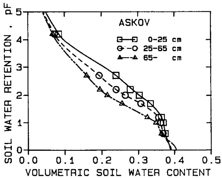
Fig. 11-2 Retention curves for Askov soil.
